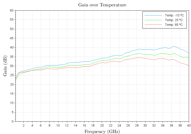
Figure 3: ERZ-HPA-0020-4000-20 Gain Vs Temperature
