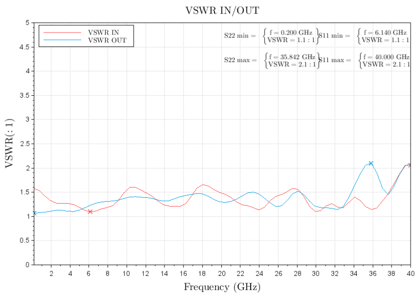
Figure 5: ERZ-HPA-0050-4000-12 Input & Output Matching
