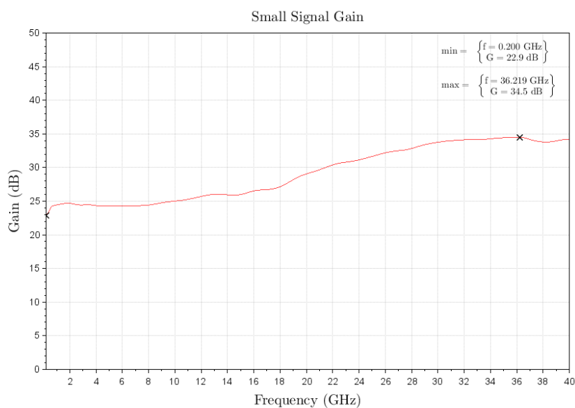
Figure 2: ERZ-HPA-0020-4000-20 Small Signal Gain
