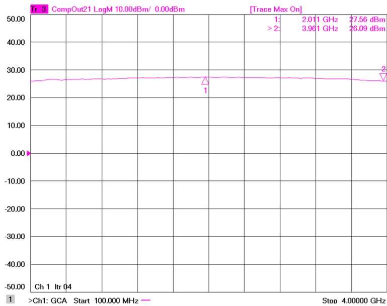
Figure 1: ERZ-HPA-0010-0400-25 P1dB
