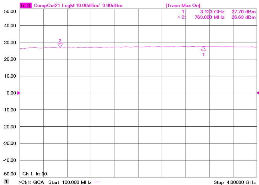
Figure 1: ERZ-HPA-0010-0400-25-E P1dB
