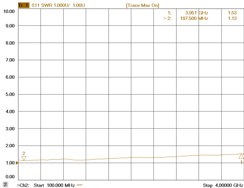
Figure 4: ERZ-HPA-0010-0400-25-E Input Matching
