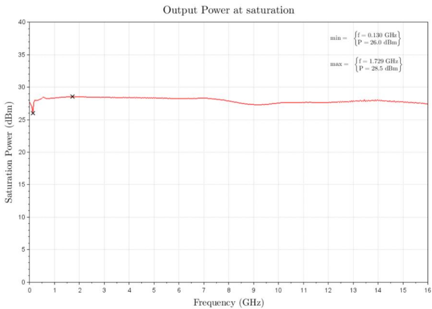
Figure 1: ERZ-HPA-0000-1200-26 Output Power at Psat
