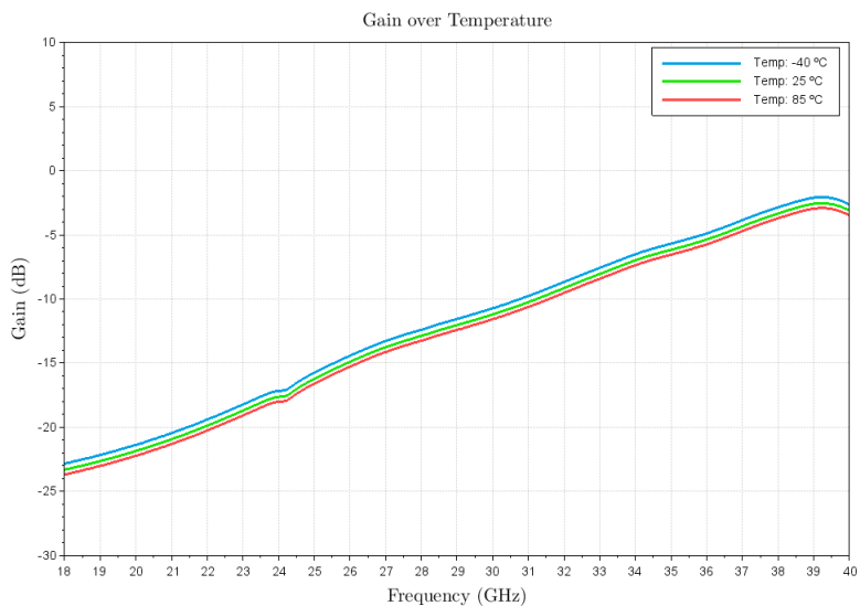
Figure 2: ERZ-EQU-1800-4000-30 Small Signal Gain
