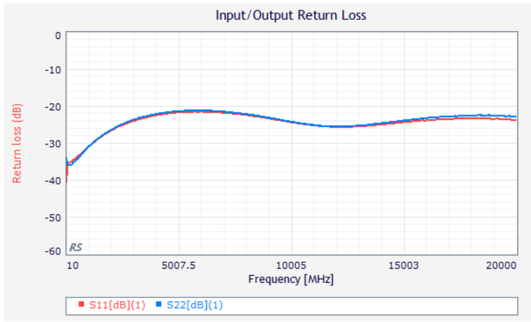
Figure 3: ERZ-EQU-0000-2000-20 Input & Output Return Loss
