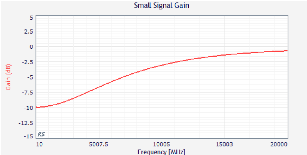
Figure 1: ERZ-EQU-0000-2000-10 Small Signal Gain
