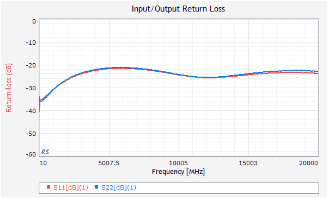
Figure 3: ERZ-EQU-0000-2000-10 Input & Output Return Loss
