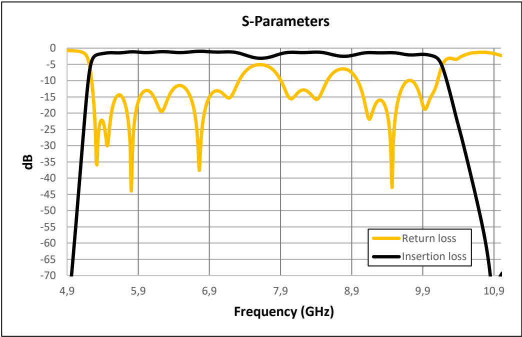
Figure 1:ERZ-BPF-0540-1000-3.1 Insertion & Return loss
