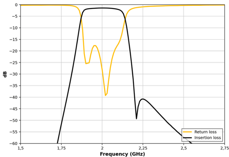
Figure 1: ERZ-BPF-0190-0210-1.8 Insertion & Return loss
