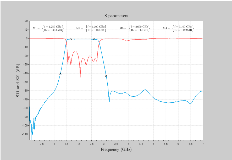
Figure 1: ERZ-BPF-0170-0260-1.5 Insertion & Return loss
