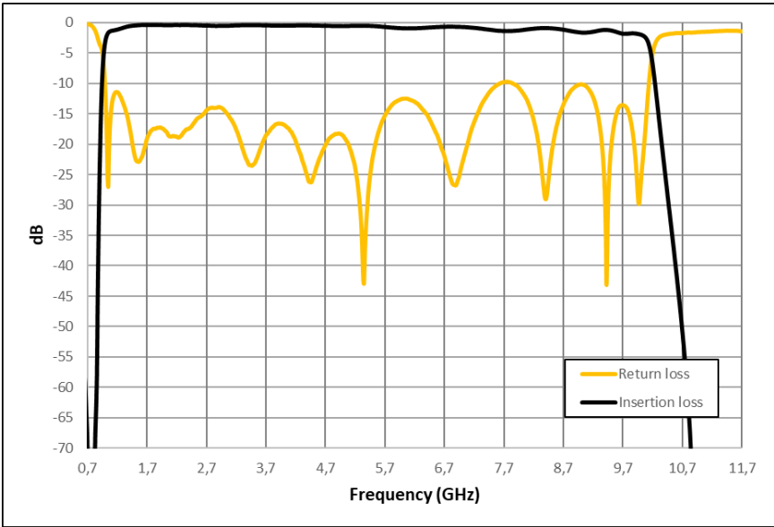
Figure 1: ERZ-BPF-0110-1000-2 Insertion & Return loss
