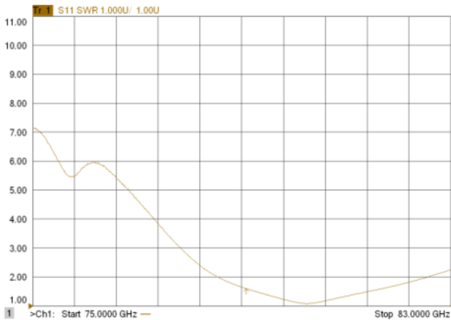
Figure 1-4: ERZ-MPA-7500-8300-13 Input Matching
