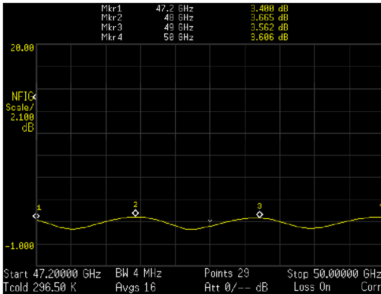
Figure 2: ERZ-LNA-4720-5140-15-4 Noise Figure
