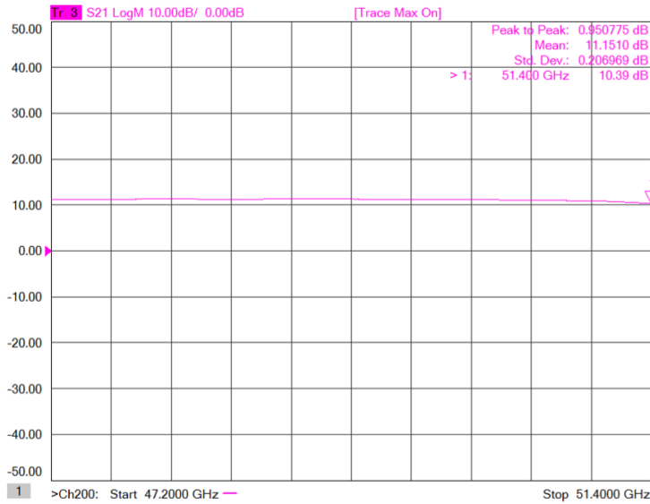
Figure 1: ERZ-LNA-4720-5140-15-4 Small Signal Gain
