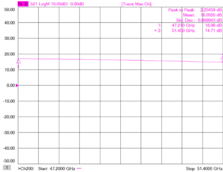
Figure 1: ERZ-LNA-4720-5140-15-3.5 Small Signal Gain
