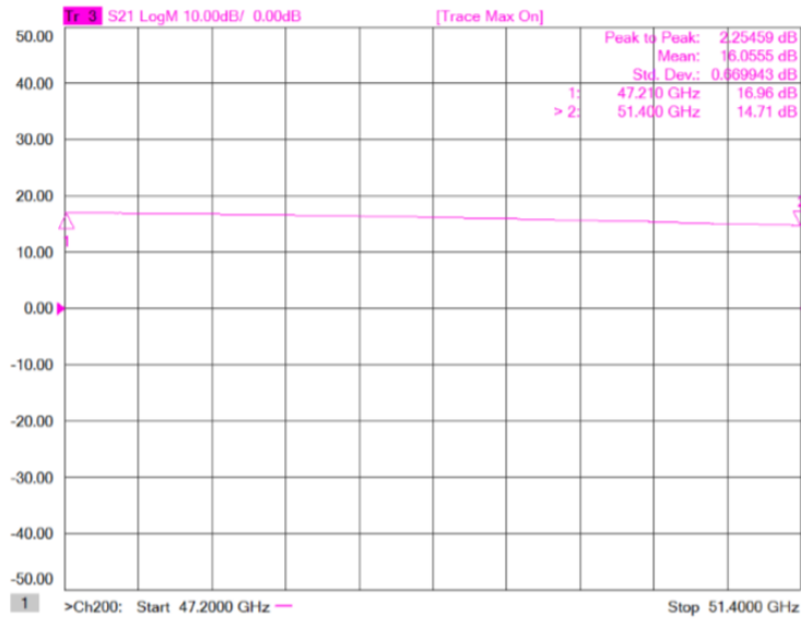
Figure 1: ERZ-LNA-4720-5140-15-3.5 Small Signal Gain
