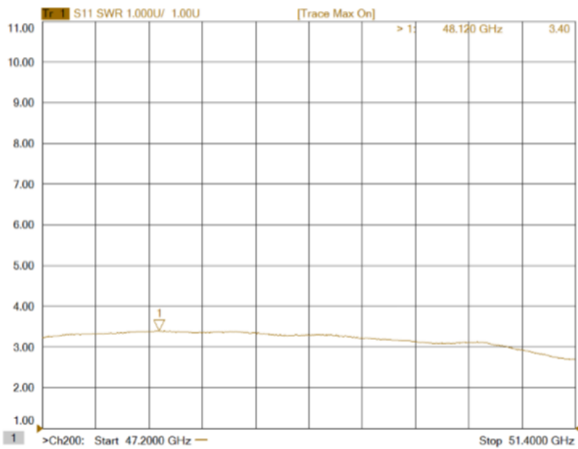
Figure 3: ERZ-LNA-4720-5140-15-3.5 Input Matching
