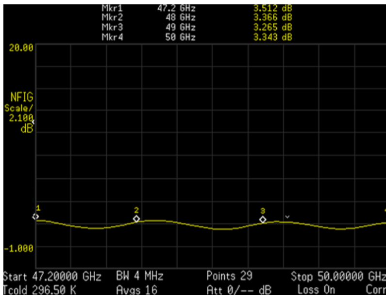
Figure 2: ERZ-LNA-4720-5140-15-3.5 Noise Figure
