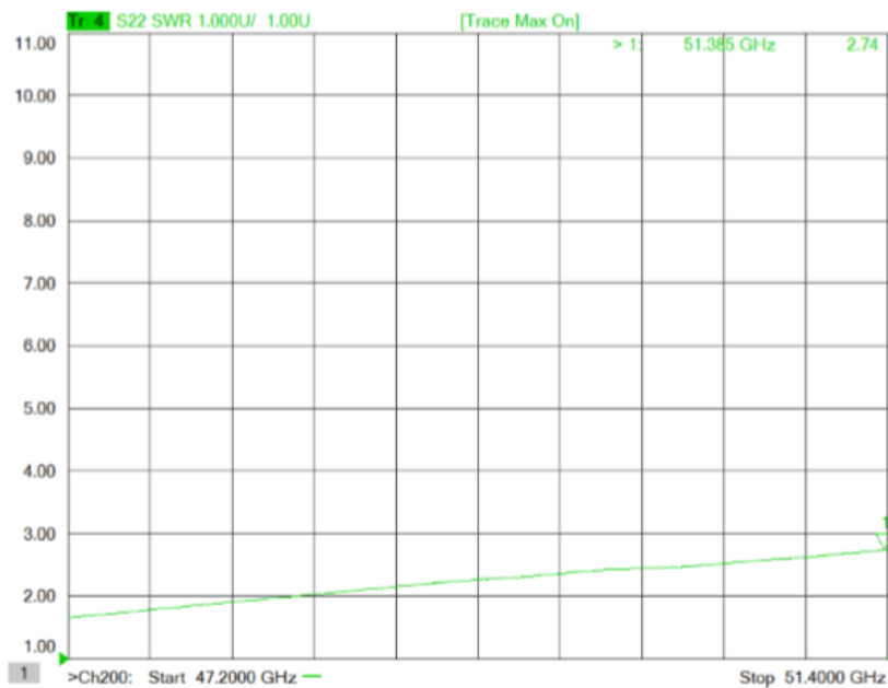
Figure 4: ERZ-LNA-4720-5140-15-3.5 Output Matching
