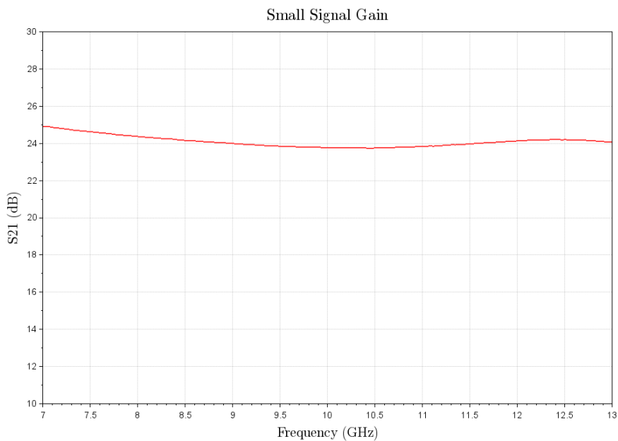
Figure 2: Figure 1: ERZ-LNA-0700-1300-22-1 Small Signal Gain
