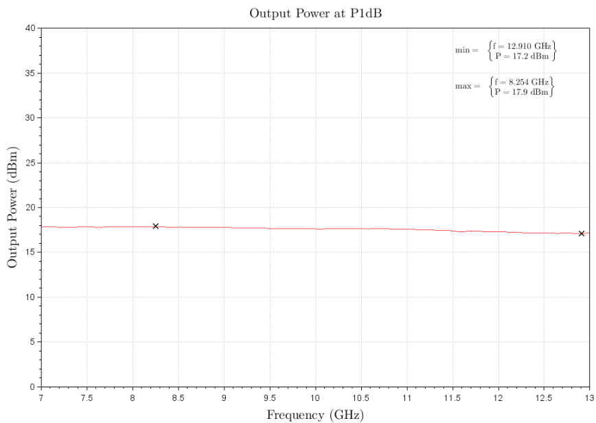
Figure 1: ERZ-LNA-0700-1300-22-1 P1dB
