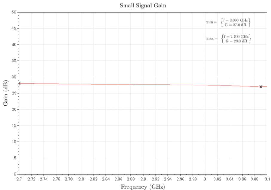
Figure 2: ERZ-LNA-0270-0310-30-0.5 Small Signal Gain
