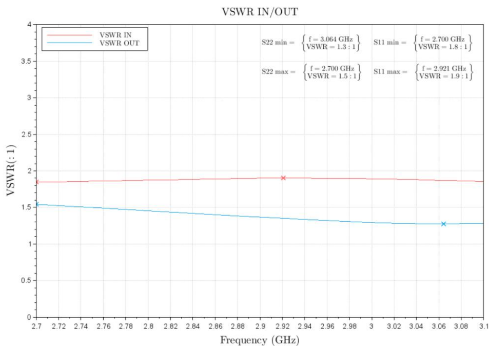
Figure 4: ERZ-LNA-0270-0310-30-0.5 Input&Output Matching
