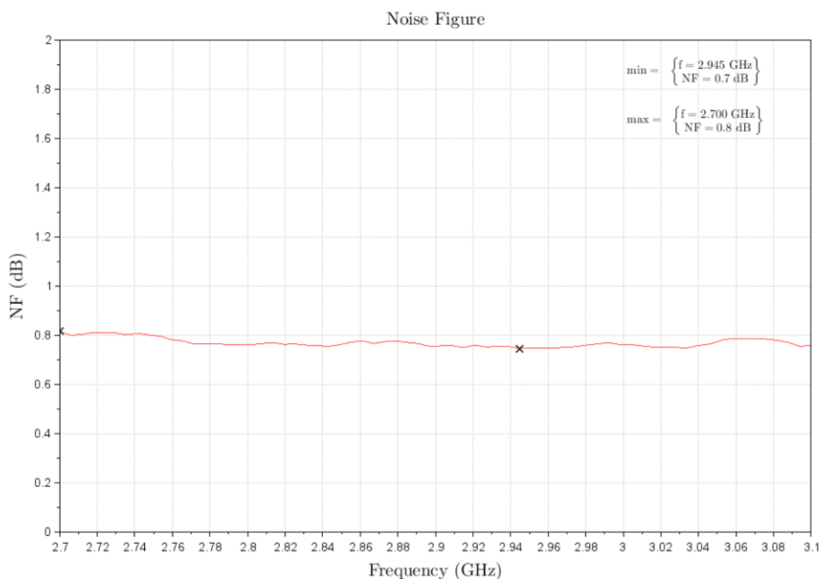
Figure 4: ERZ-LNA-0270-0310-30-0.5 Noise Figure
