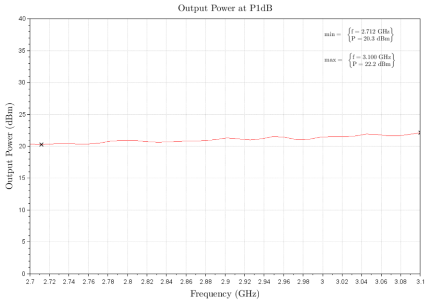
Figure 1: ERZ-LNA-0270-0310-30-0.5 P1dB
