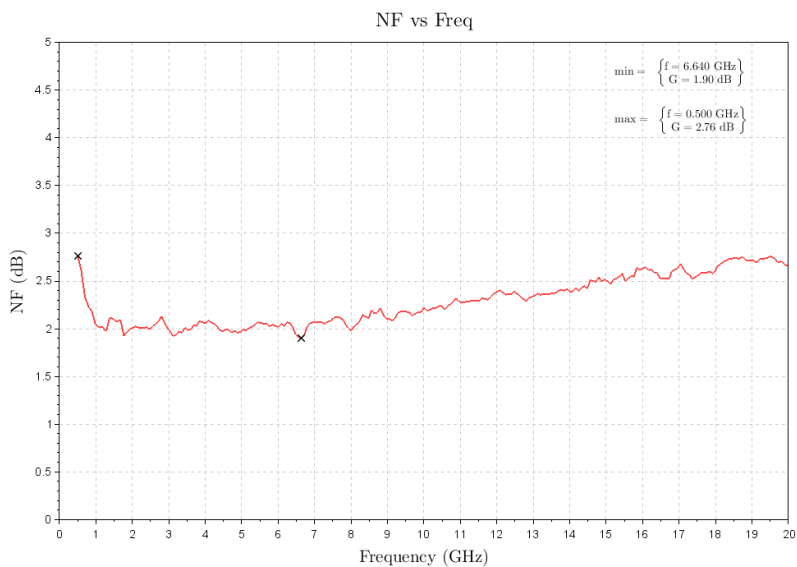
Figure 3: ERZ-LNA-0050-2000-15-2.5 Noise Figure
