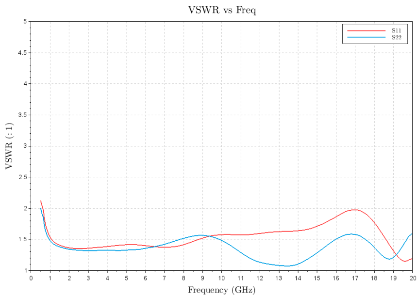
Figure 4: ERZ-LNA-0050-2000-15-2.5 Input & Output Matching
