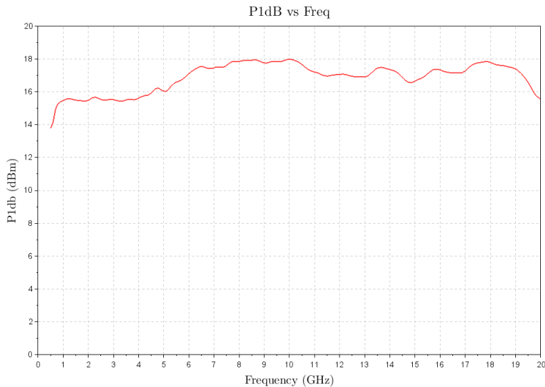
Figure 1: ERZ-LNA-0050-2000-15-2.5 P1dB
