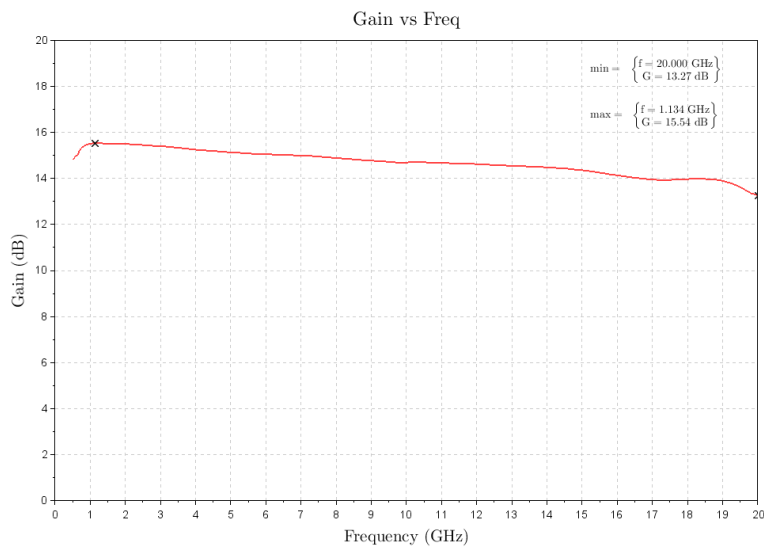
Figure 2: ERZ-LNA-0050-2000-15-2.5 Small Signal Gain
