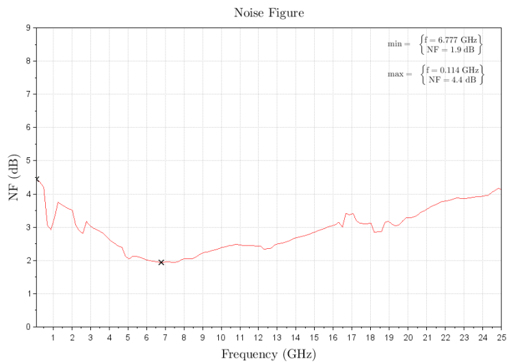
Figure 4: ERZ-LNA-0000-2500-14-2.5 Noise Figure
