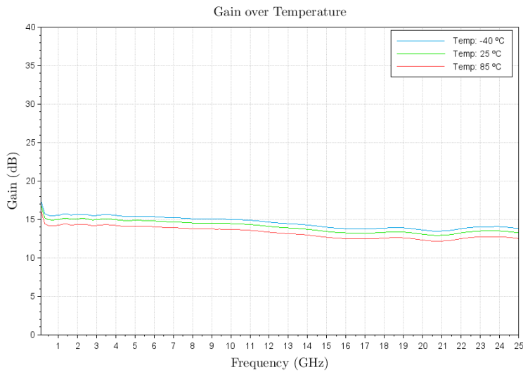
Figure 3: ERZ-LNA-0000-2500-14-2.5 Small Signal Gain
