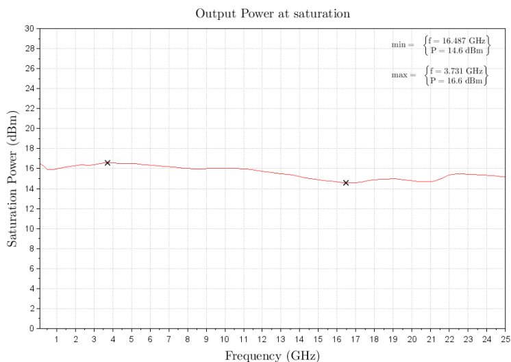
Figure 2: ERZ-LNA-0000-2500-14-2.5 Psar
