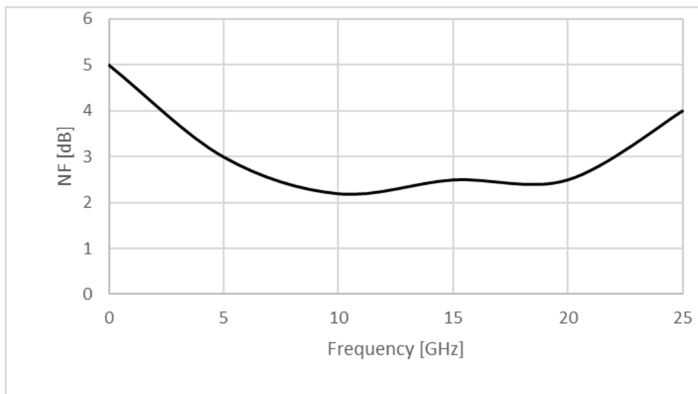
Figure 3: ERZ-LNA-0000-2500-14-2.5 Noise Figure
