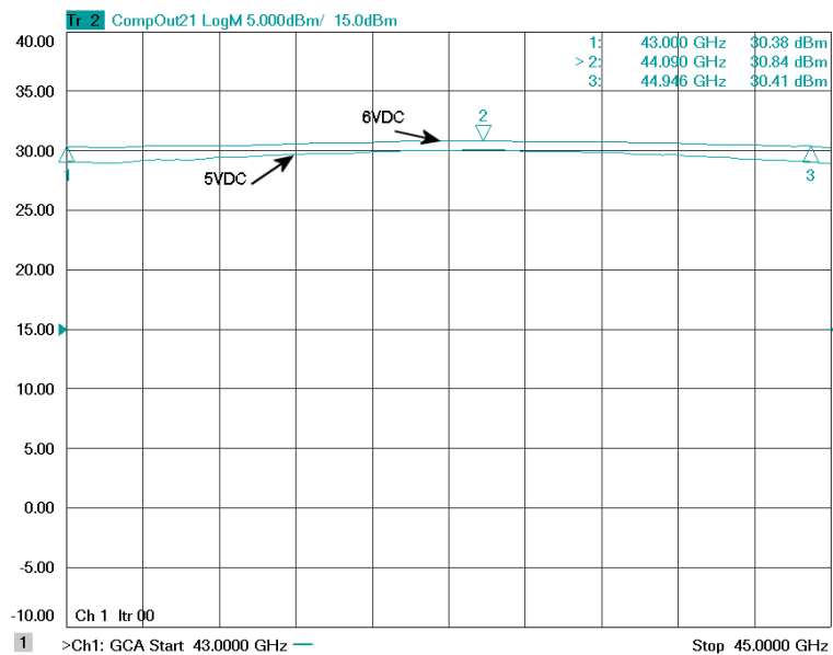
Figure 1-1: ERZ-HPA-4300-4600-30 P1dB
