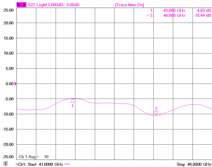
Figure 1-5: ERZ-HPA-4300-4600-30 Output Matching
