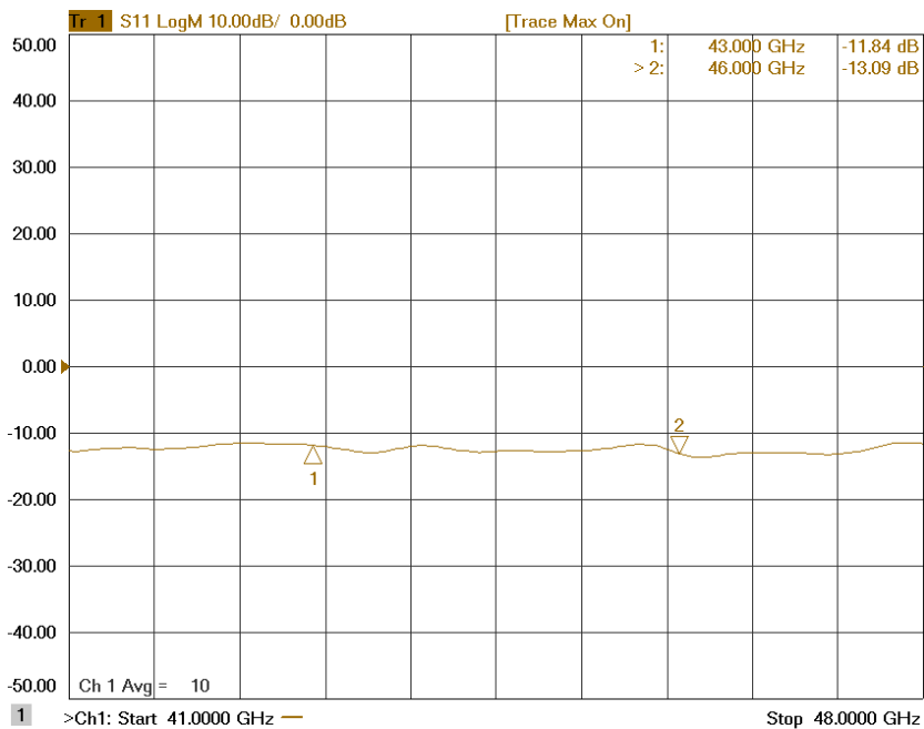
Figure 1-4: ERZ-HPA-4300-4600-30 Input Matching
