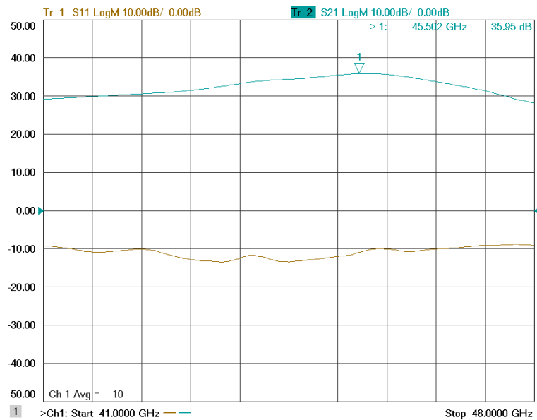
Figure 1-2: ERZ-HPA-4300-4600-30 Small Signal Gain
