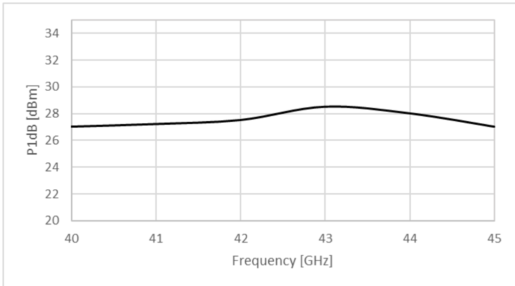
Figure 1: ERZ-HPA-4000-4500-28-E P1dB
