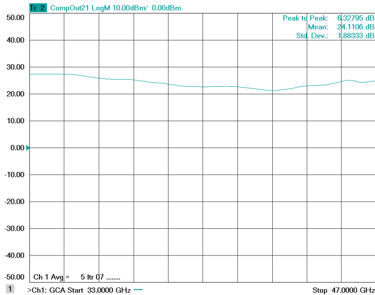
Figure 1: ERZ-HPA-3300-4700-24 Psat
