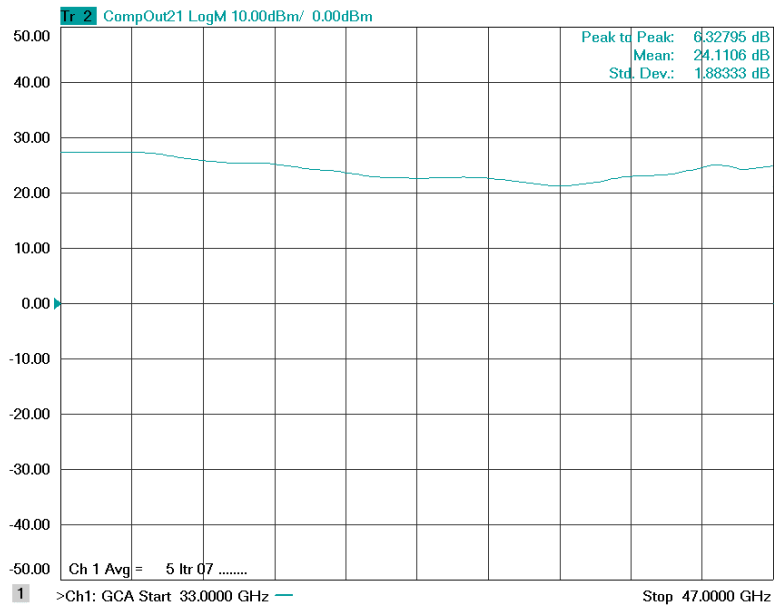
Figure 1: ERZ-HPA-3300-4700-24 Psat
