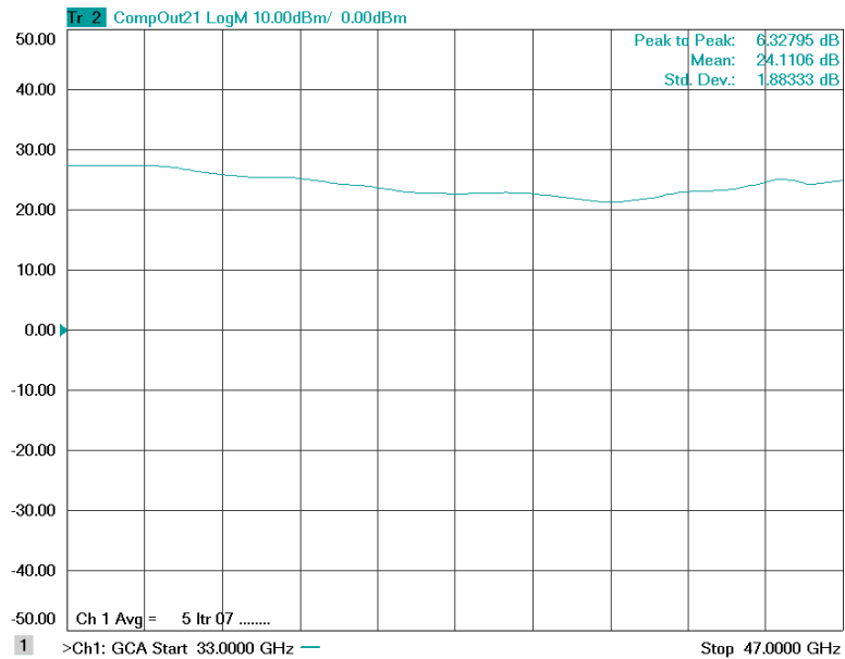
Figure 1: ERZ-HPA-3300-4700-24-E Psat
