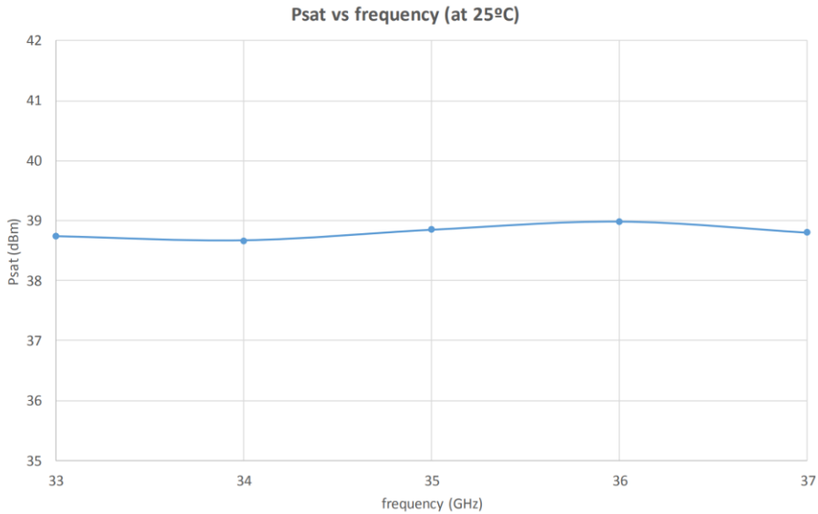
Figure 1: ERZ-HPA-3300-3700-38 Psat
