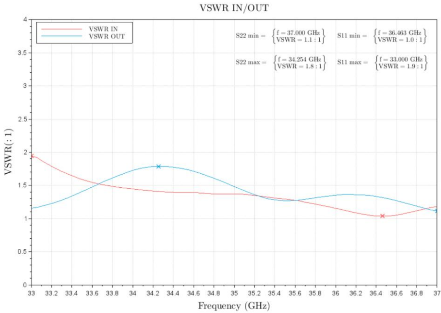
Figure 3: ERZ-HPA-3300-3700-38 Input and Output Matching
