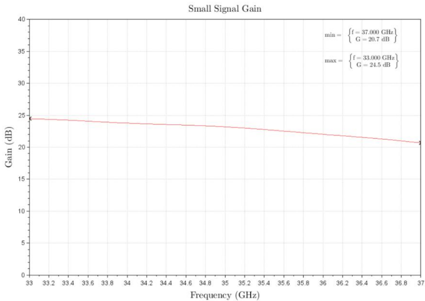
Figure 2: ERZ-HPA-3300-3700-38 Small Signal Gain
