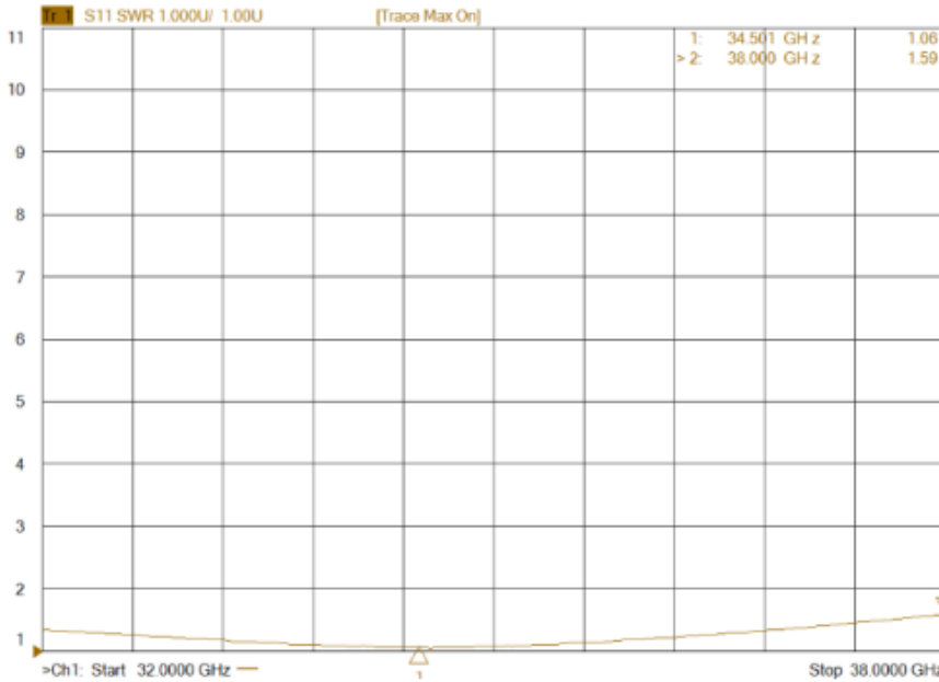
Figure 3: ERZ-HPA-3200-3800-40 VSWR IN
