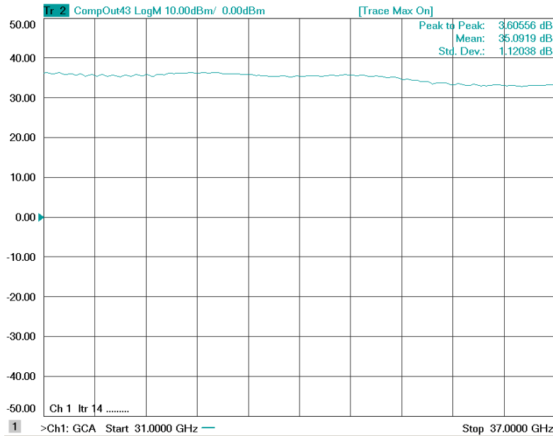
Figure 1: ERZ-HPA-3100-3700-33 Psat
