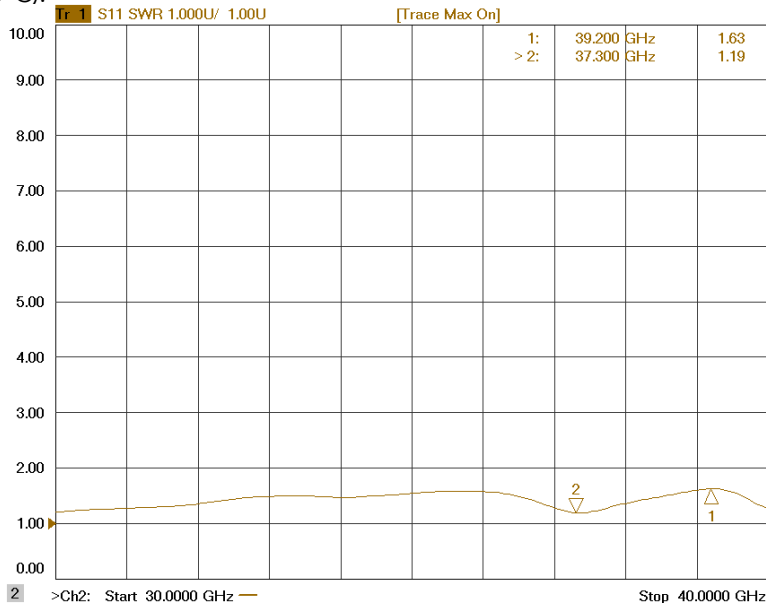
Figure 1-4: ERZ-HPA-3000-4000-32-E Input Matching
