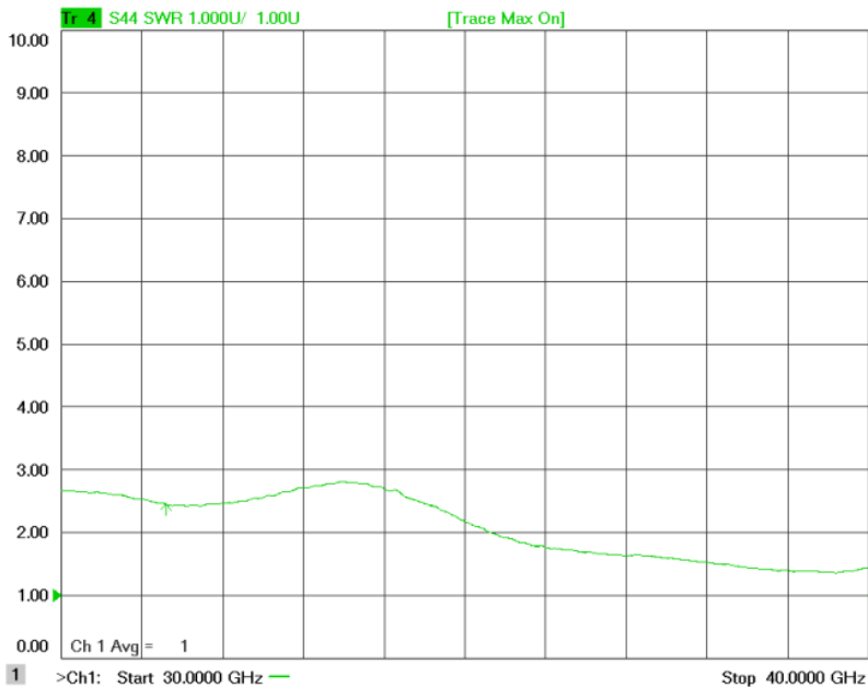
Figure 1-5: ERZ-HPA-3000-4000-32-E Output Matching
