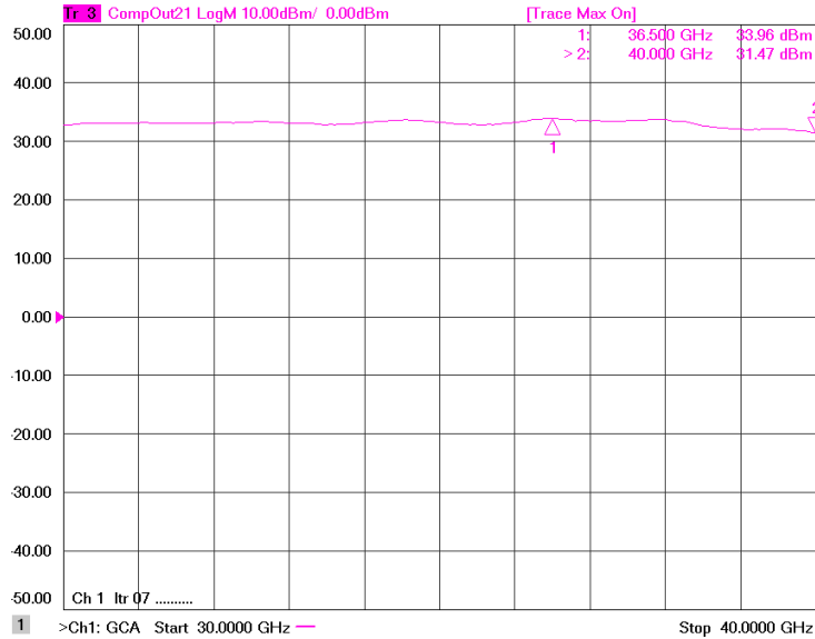
Figure 1: ERZ-HPA-3000-4000-32-E Psat
