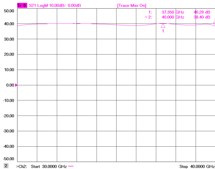
Figure 2: ERZ-HPA-3000-4000-32-E Small Signal Gain
