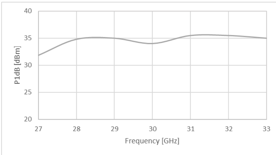
Figure 1: ERZ-HPA-2800-3300-33 P1dB
