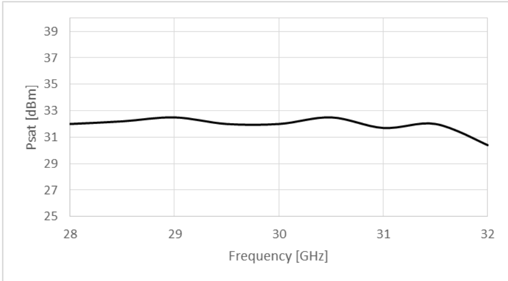
Figure 1: ERZ-HPA-2800-3200-32 P1dB
