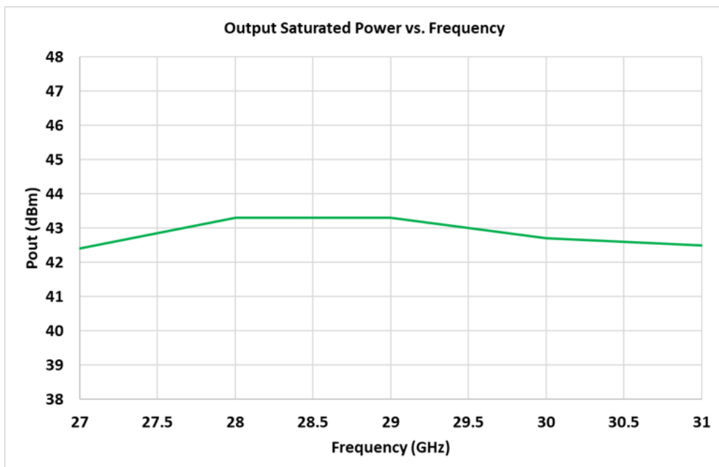
Figure 1: ERZ-HPA-2700-3100-43-P Psat
