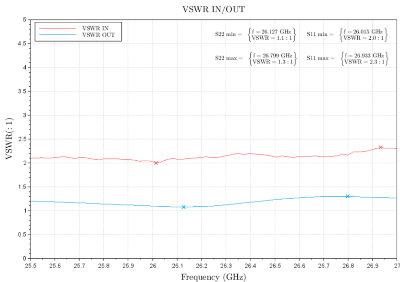
Figure 4: ERZ-HPA-2550-2700-37 Input & Output Matching
