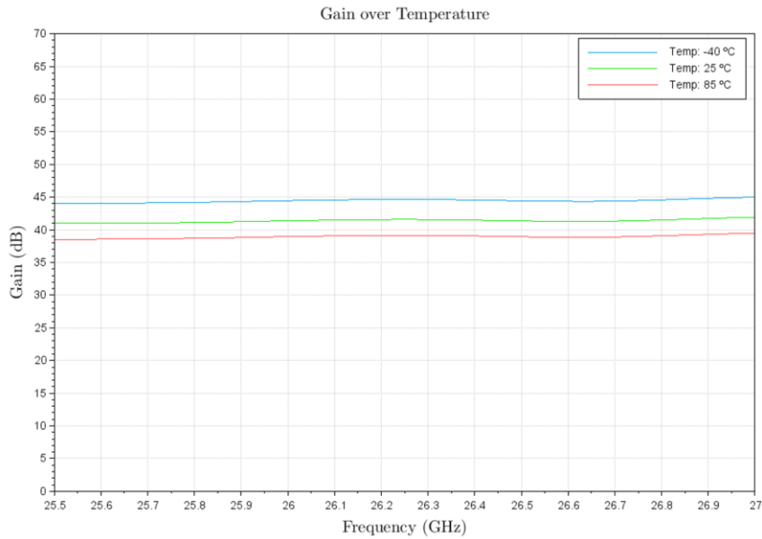
Figure 3: ERZ-HPA-2550-2700-37 Small Signal Gain
