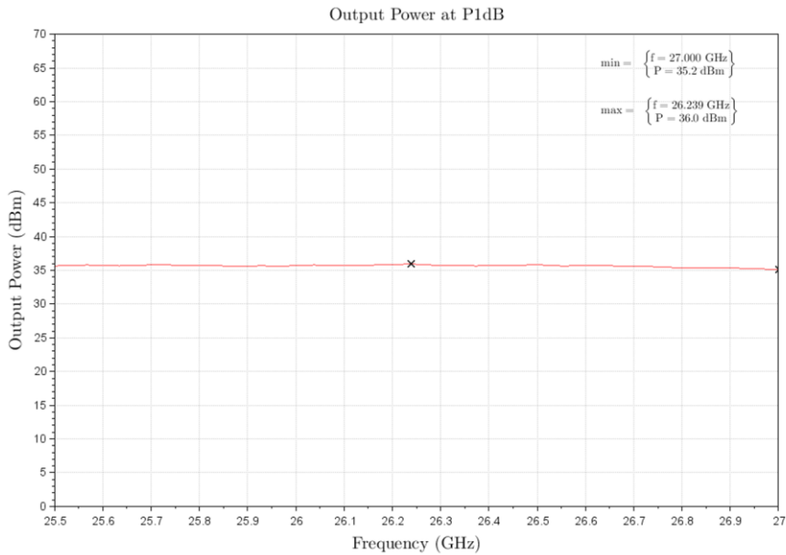
Figure 1: ERZ-HPA-2550-2700-37 P1dB
