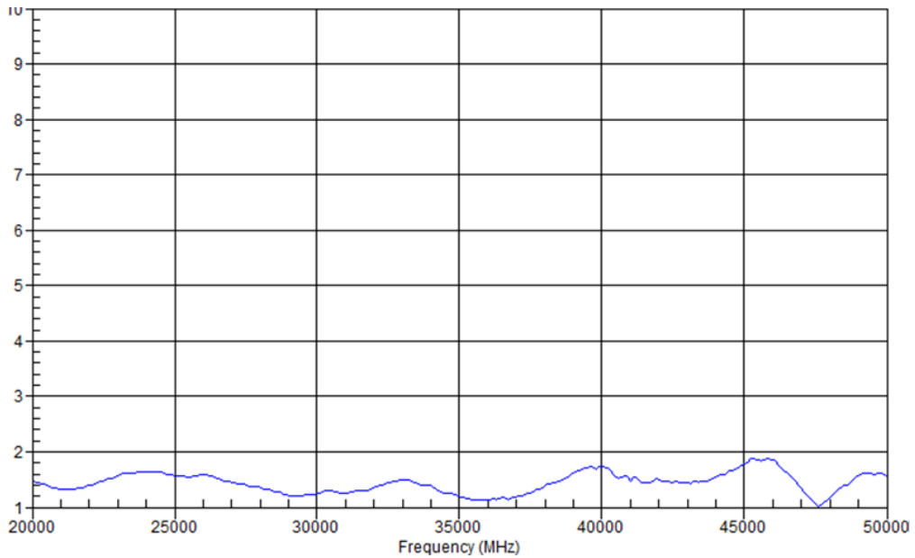
Figure 3: ERZ-HPA-2400-5000-28 Input VSWR
