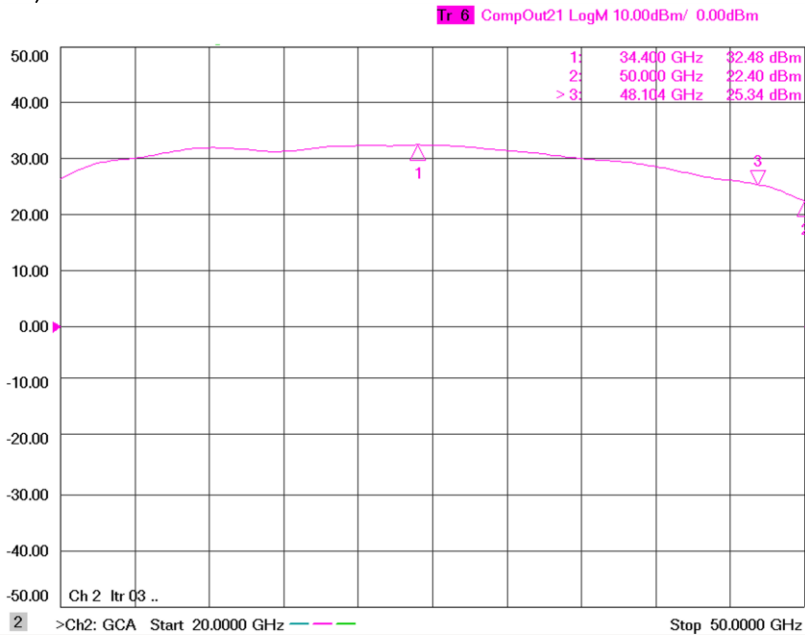
Figure 1: ERZ-HPA-2400-5000-28 Psat
