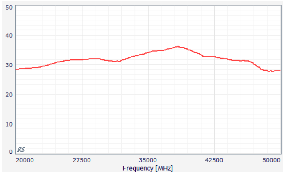
Figure 2: ERZ-HPA-2400-5000-28 Small Signal Gain
