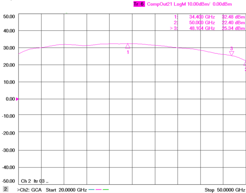
Figure 1: ERZ-HPA-2400-5000-28 Psat
