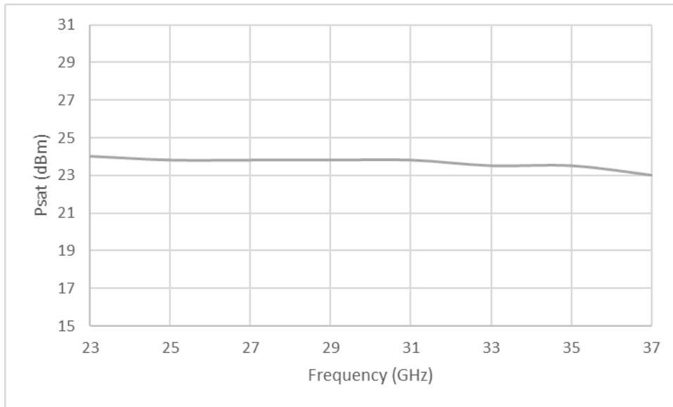
Figure 1: ERZ-HPA-2300-3700-25 Psat
