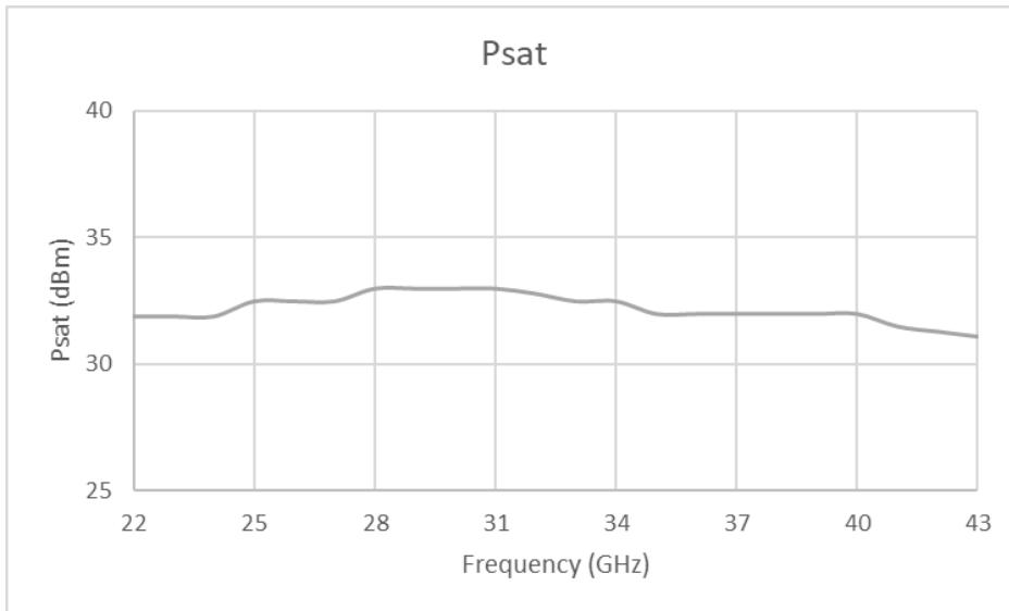
Figure 1: ERZ-HPA-2200-4300-32 Psat
