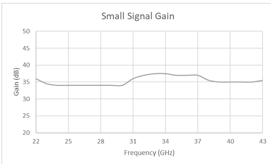
Figure 2: ERZ-HPA-2200-4300-32 Small Signal Gain
