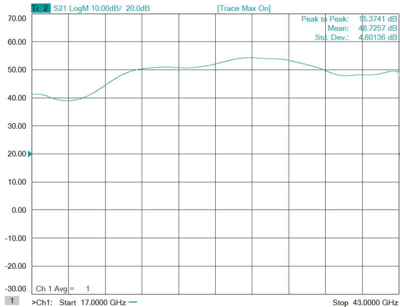
Figure 2: ERZ-HPA-1700-4300-22-E Small Signal Gain
