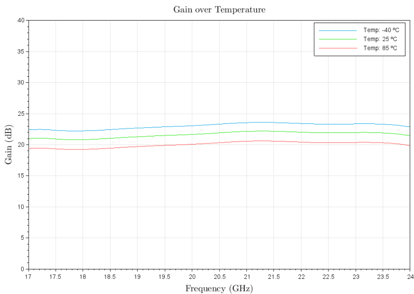
Figure 2: ERZ-HPA-1700-2400-34 Small Signal Gain
