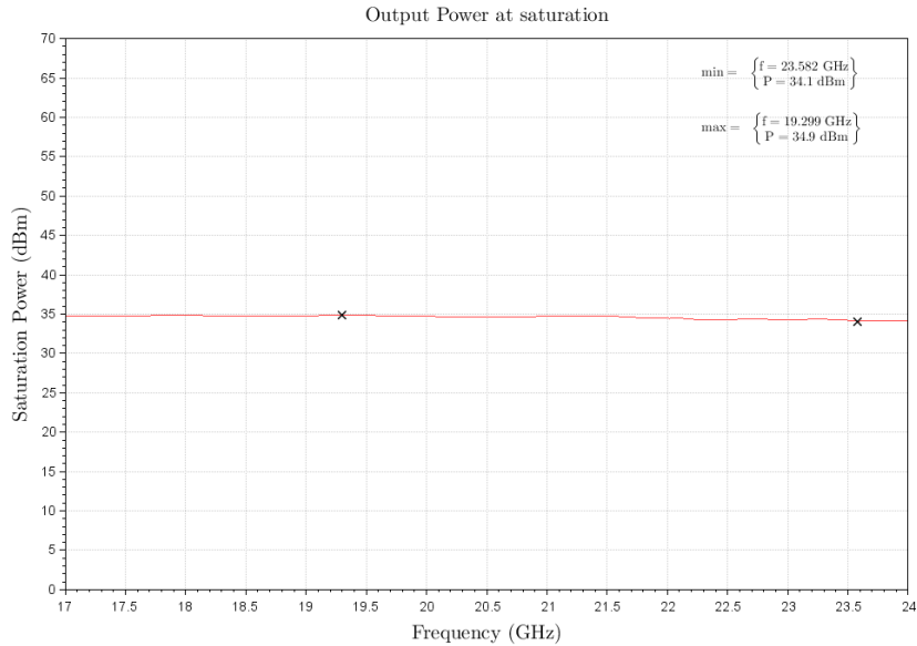
Figure 1: ERZ-HPA-1700-2400-34 Psat
