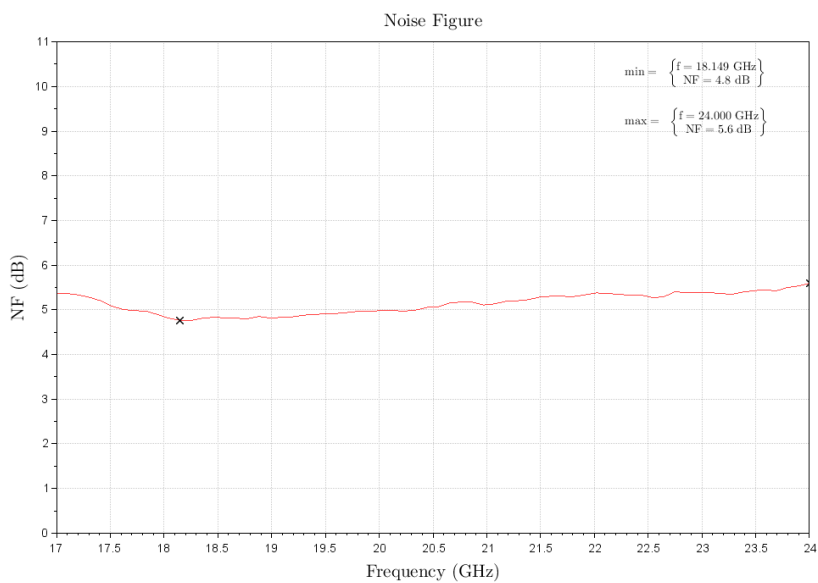
Figure 4: ERZ-HPA-1700-2400-34 Noise Figure
