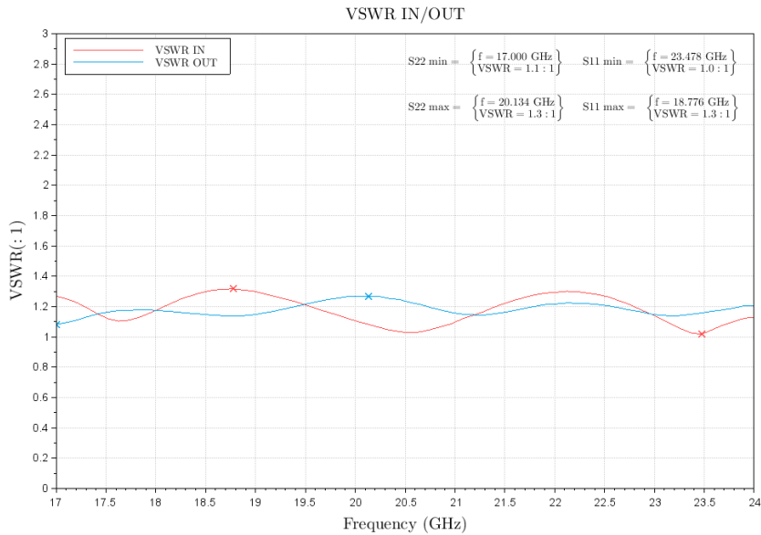
Figure 3: ERZ-HPA-1700-2400-34 VSWR IN/OUT
