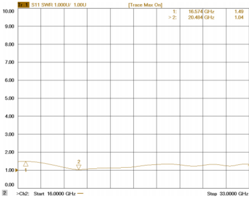
Figure 3: ERZ-HPA-1600-3300-24 Input Matching
