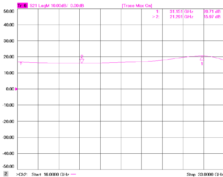
Figure 2: ERZ-HPA-1600-3300-24 Small Signal Gain
