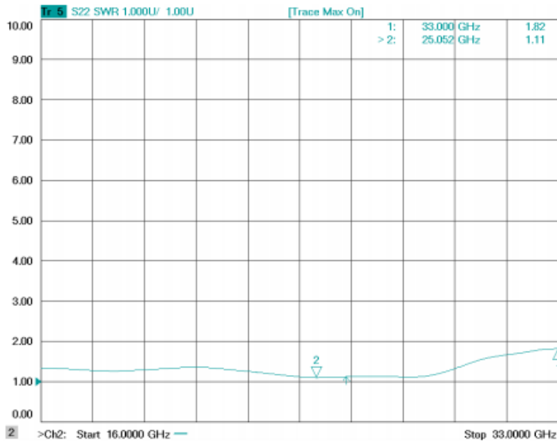
Figure 4: ERZ-HPA-1600-3300-24 Output Matching
