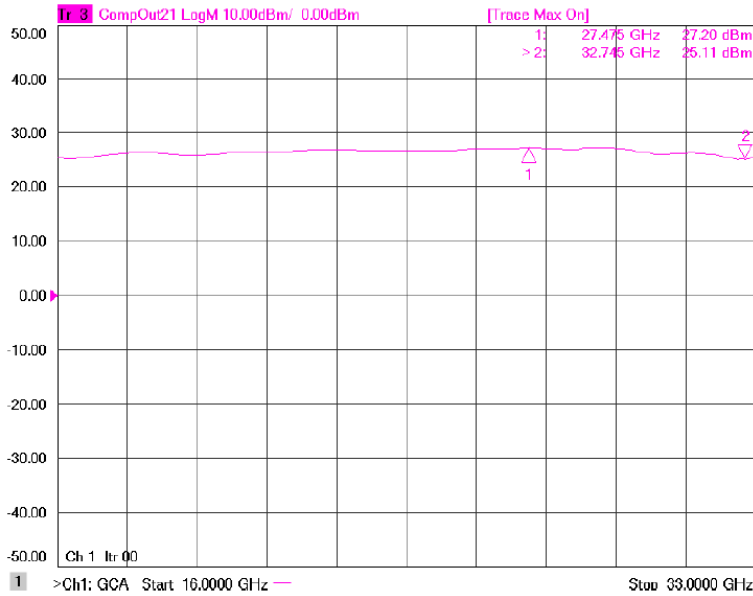
Figure 1: ERZ-HPA-1600-3300-24 Psat
