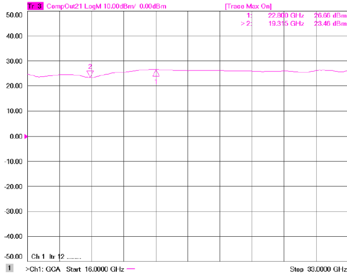
Figure 1: ERZ-HPA-1600-3300-24-E Psat
