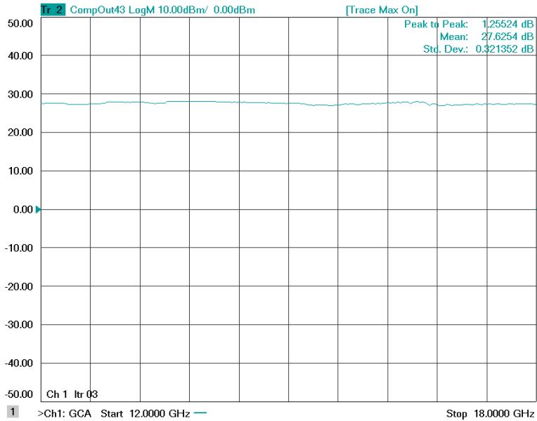
Figure 1-1: ERZ-HPA-1200-1800-27 P1dB
