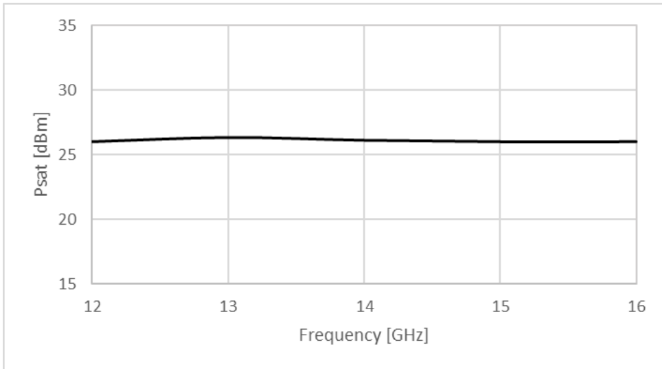
Figure 1: ERZ-HPA-1200-1600-26 Psat
