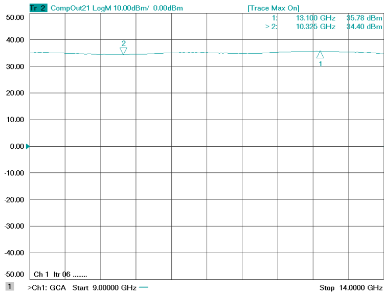
Figure 1: ERZ-HPA-0900-1400-34 Psat
