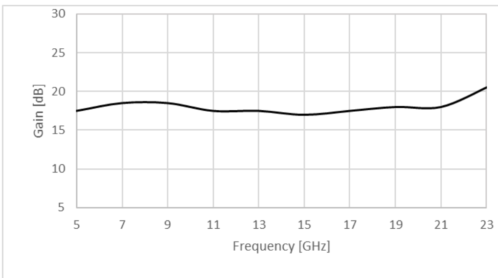
Figure 2: ERZ-HPA-0500-2300-20 Small Signal Gain
