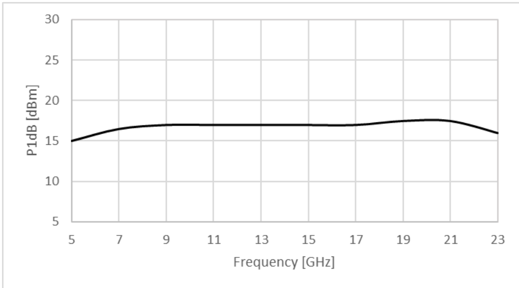
Figure 1: ERZ-HPA-0500-2300-20 P1dB
