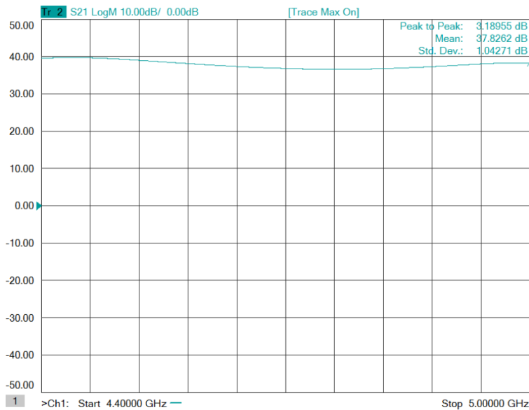
Figure 2: ERZ-HPA-0440-0500-40 Small Signal Gain
