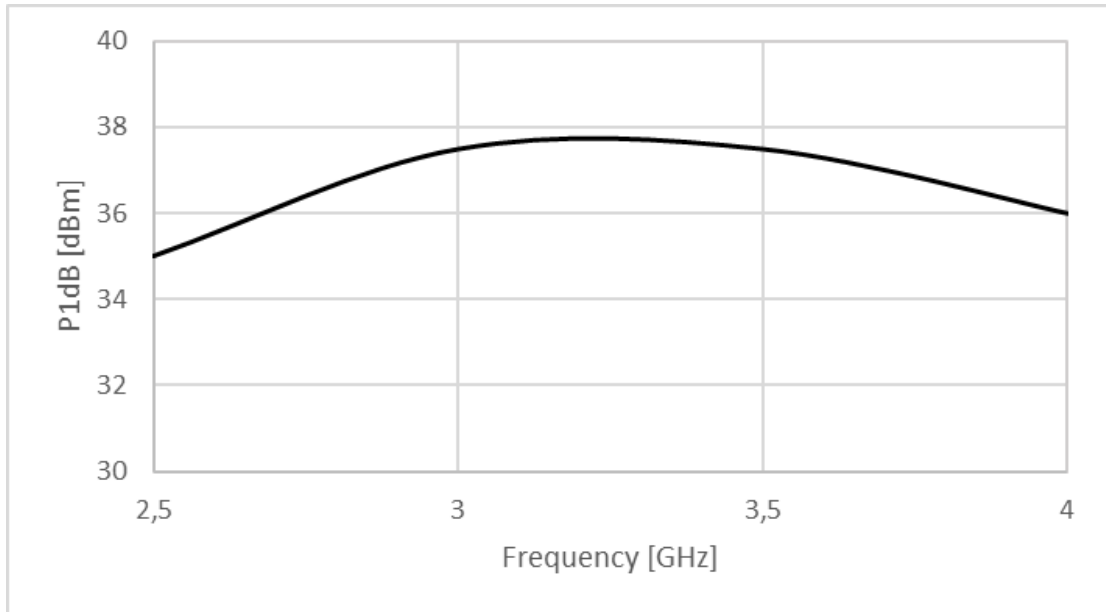
Figure 1: ERZ-HPA-0250-0400-35 P1dB
