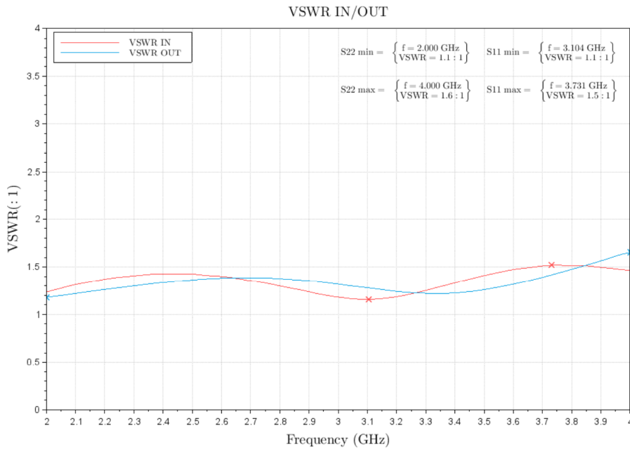
Figure 3: ERZ-HPA-0200-0400-24 Input & Output Matching
