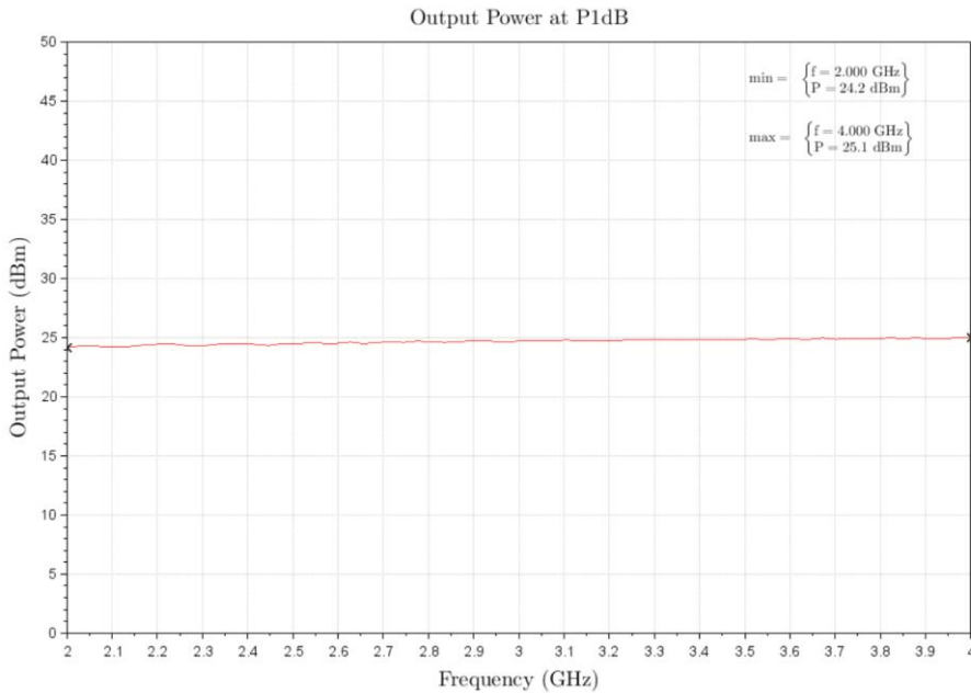
Figure 1: ERZ-HPA-0200-0400-24 P1dB
