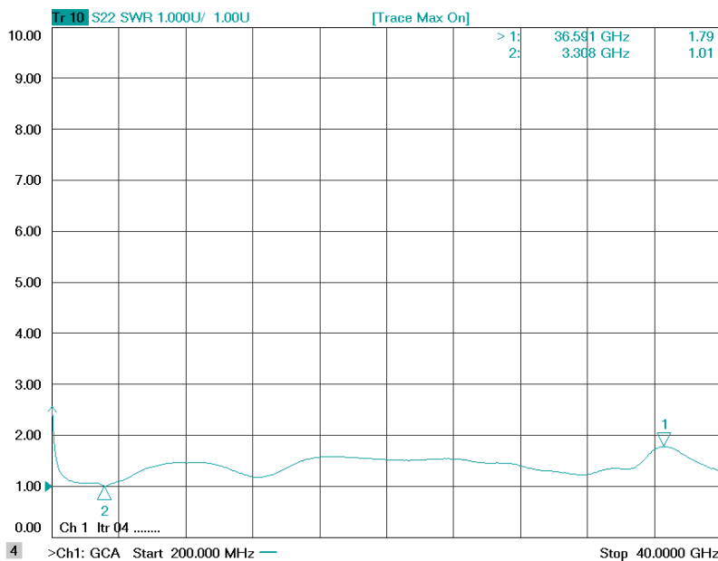
Figure 5: ERZ-HPA-0050-4000-12 Output Matching
