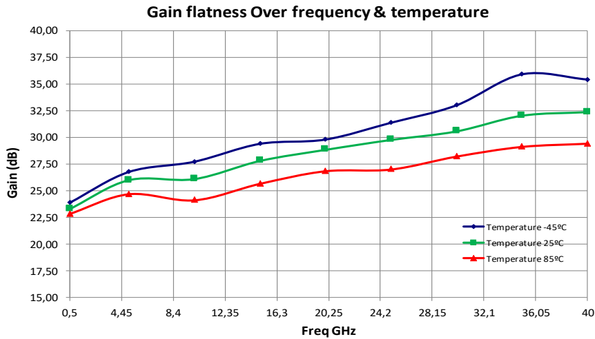
Figure 3: ERZ-HPA-0050-4000-12 Small Signal Gain Vs Temperature
