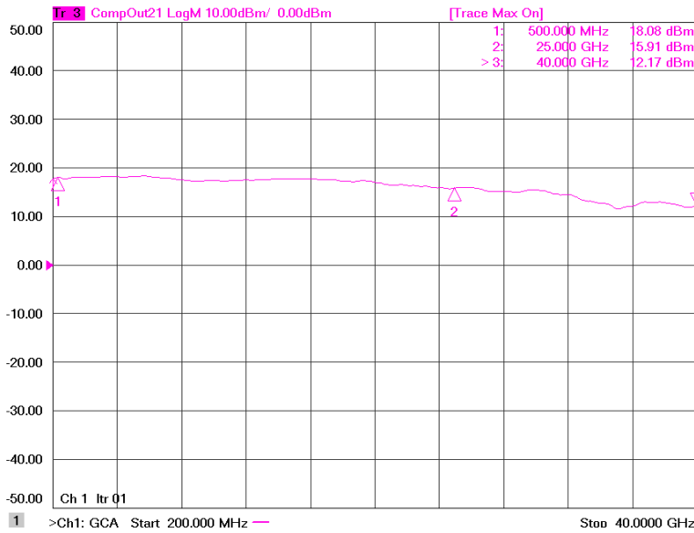
Figure 1: ERZ-HPA-0050-4000-12 P1dB
