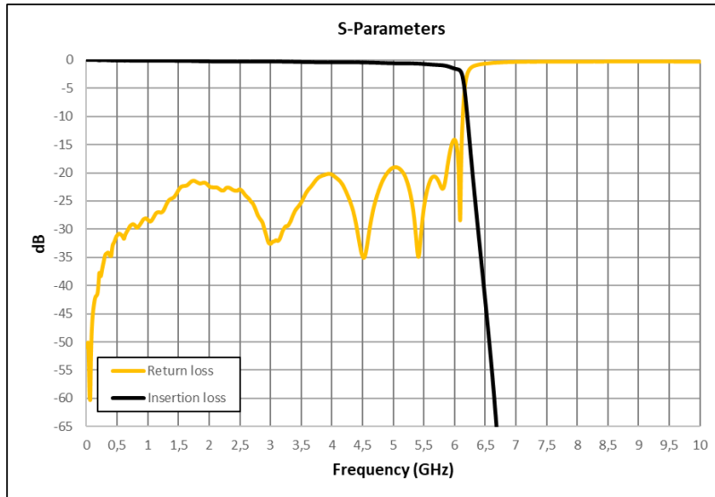
Figure 1:ERZ-LPF-0000-0610-1.6 Insertion & Return loss
